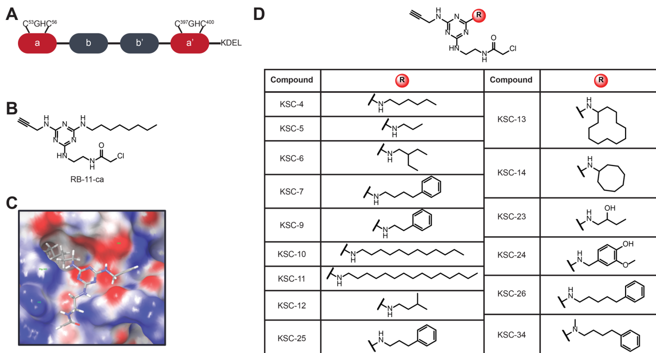
Figure 1. Domain organization of PDIA1 and chemical structures of PDIA1 inhibitors. (A) PDIA1 comprises two active-site a-type domains that contain a CGHC active-site motif, together with two b domains implicated in substrate recognition and binding. (B) Chemical structure of RB-11-ca, a previously reported a-site inhibitor of PDIA1. RB-11-ca contains a central triazine scaffold, a chloroacetamide reactive group for covalent cysteine modification, an alkyne bioorthogonal handle for CuAAC, and an octylamine diversity element. (C) Predicted binding pose of RB-11-ca in the a domain active site of PDIA1 by the covalent docking algorithm from Schrodinger, Inc. (D) Structures of second-generation PDIA1 inhibitors obtained by varying the diversity element of RB-11-ca.
