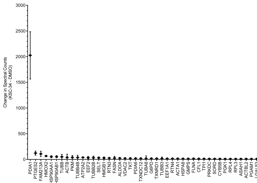
Figure 4. Evaluation of proteome-wide selectivity of KSC-34. Mass spectrometry analysis of proteins enriched in KSC-34-treated ( 5 \mu\text{M} ) and dimethyl sulfoxide-treated MCF-7 cells. The spectral count differences between KSC-34-treated and dimethyl sulfoxide-treated samples are plotted for all proteins identified (Table S2). Error bars indicate the SD for two experiments.
