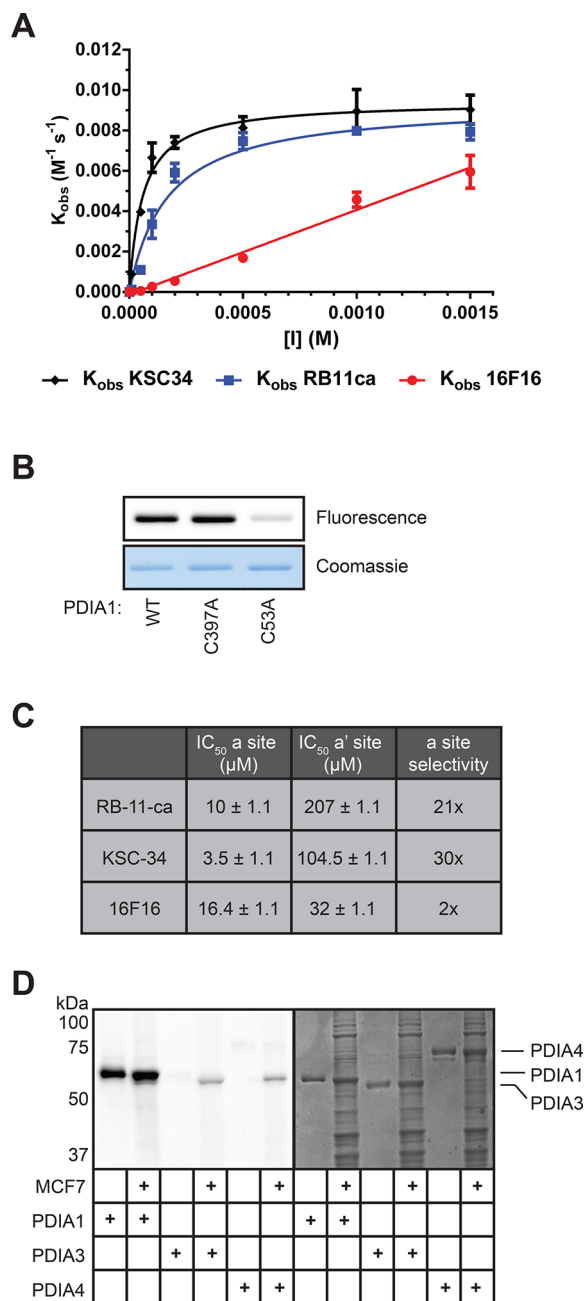
Figure 3. Evaluation of the potency and selectivity of KSC-34. (A) Concentration- and time-dependent inhibition of PDIA1 by KSC-34, RB-11-ca, and 16F16. PDIA1 reductase activity was measured using an insulin reduction assay in a 100 μL reaction volume containing 0.5 μM PDIA1, 0.16 mM insulin, and 1 mM DTT in assay buffer. The turbidity of the insulin solution was measured over time at various concentrations and preincubation times with KSC-34. Error bars represent the SD from two experiments. (B) Labeling of wild-type PDIA1, C397A, and C53A by KSC-34. Each recombinant PDIA1 protein (50 μg/mL) was incubated with KSC-34 (5 μM) for 1 h and subjected to CuAAC with TAMRA-azide prior to in-gel fluorescence. (C) Active-site selectivity for KSC-34, RB-11-ca, and 16F16. KSC-34 was found to have a 30-fold selectivity for the a domain over the a' domain, compared to RB-11-ca, which exhibited a 21-fold selectivity, and 16F16, which exhibited a 2-fold selectivity. The error is calculated by PRISM as ±SEM from three experiments. (D) PDI isoform selectivity. KSC-34 was found to covalently modify only PDIA1, over PDIA3 and PDIA4, two closely related family members. Fluorescent bands in cell lysate lanes for PDIA3 and PDIA4 samples represent endogenous PDIA1 protein.
