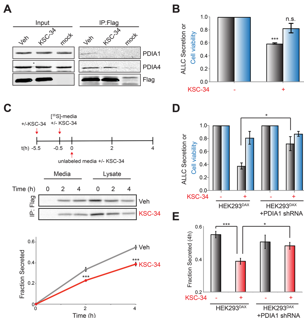
Figure 6. KSC-34 reduces the rate of secretion of destabilized ALLC from mammalian cells. (A) Immunoblot of anti-FLAG IPs of lysates prepared from HEK293 DAX cells transiently transfected with FT ALLC and pretreated for 1 h with vehicle or KSC-34 (40 μM). Cells were cross-linked for 30 min with DSP (500 μM) prior to lysis. Mock transfected cells are included as a control. (B) Graph showing secreted FT ALLC (gray) and viability (blue) of HEK293 Trex cells stably expressing FT ALLC pretreated for 4 h with KSC-34 (40 μM). The medium was conditioned for 2 h in the presence or absence of KSC-34 (40 μM) prior to quantification of secreted FT ALLC by an enzyme-linked immunosorbent assay (ELISA). Viability was measured following conditioning of the medium with Cell Titer Glo. All data are normalized to vehicle-treated cells. Error bars show the SEM for three experiments. *** p < 0.005. (C) Representative autoradiogram and quantification of the fraction of 35 S-labeled FT ALLC secreted from HEK293 DAX cells using the experimental paradigm shown. Experiments were performed in the absence or presence of KSC-34 (40 μM) added 1 h prior to labeling and then again throughout the experiment. The fraction secreted was calculated as described in the Supporting Information. 44 Error bars show the SEM for four experiments. *** p < 0.005. (D) Graph showing secreted FT ALLC (gray) and viability (blue) of HEK293 DAX cells transiently expressing FT ALLC pretreated for 4 h with KSC-34 (40 μM). HEK293 DAX cells stably expressing PDIA1 shRNA are indicated. The medium was conditioned for 2 h in the presence or absence of KSC-34 (40 μM) prior to quantification of secreted FT ALLC by an ELISA. Viability was measured following conditioning of the medium with Cell Titer Glo. All data are normalized to vehicle-treated controls. Error bars show the SEM for three experiments. * p < 0.05. (E) Graph showing the fraction of 35 S-labeled FT ALLC secreted at 4 h from HEK293 DAX cells transiently transfected with FT ALLC quantified using the same experimental paradigm shown in panel C. HEK293 DAX cells stably expressing PDIA1 shRNA are indicated. Experiments were performed in the absence or presence of KSC-34 (40 μM) added 1 h prior to labeling and then again throughout the experiment. Error bars show the SEM for four experiments. * p < 0.05; *** p < 0.005.
