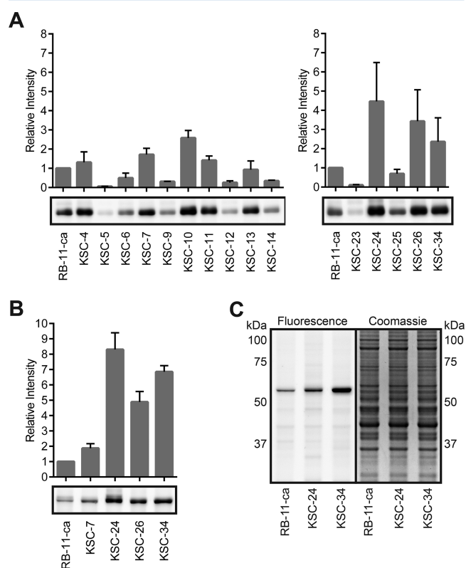
Figure 2. Characterization of PDIA1 second-generation library members. (A) Library members (5 \mu\text{M} ) were incubated with purified recombinant PDIA1 (50 \mu\text{g}/\text{mL} ) in PBS, and protein labeling by each compound was evaluated after CuAAC-mediated incorporation of a TAMRA fluorophore, sodium dodecyl sulfate–polyacrylamide gel electrophoresis, and in-gel fluorescence (complete gel images provided in Figure S1 ). Library members with potency equal to or greater than that of RB-11-ca progressed to the next step of the assay. (B) In-gel fluorescence studies of library members (5 \mu\text{M} ) incubated with MCF-7 cell lysate (2 mg/mL) to assess potency and selectivity for endogenous PDIA1 in a complex proteome (complete gel images provided in Figure S3 ). (C) To assess cell permeability as well as selectivity of the library, probes (5 \mu\text{M} ) were incubated with MCF-7 cells for 3 h at 37 °C. Following cell lysis and in-gel fluorescence, KSC-34 was found to be ~8-fold more potent than the lead compound, RB-11-ca, in whole cells against PDIA1 (left). A Coomassie gel is presented in the right panel to show normalized protein abundance. Fluorescence intensity quantified by ImageJ (National Institutes of Health, Bethesda, MD). All data are normalized to RB-11-ca, and error bars represent the standard deviation (SD) for three experiments.
