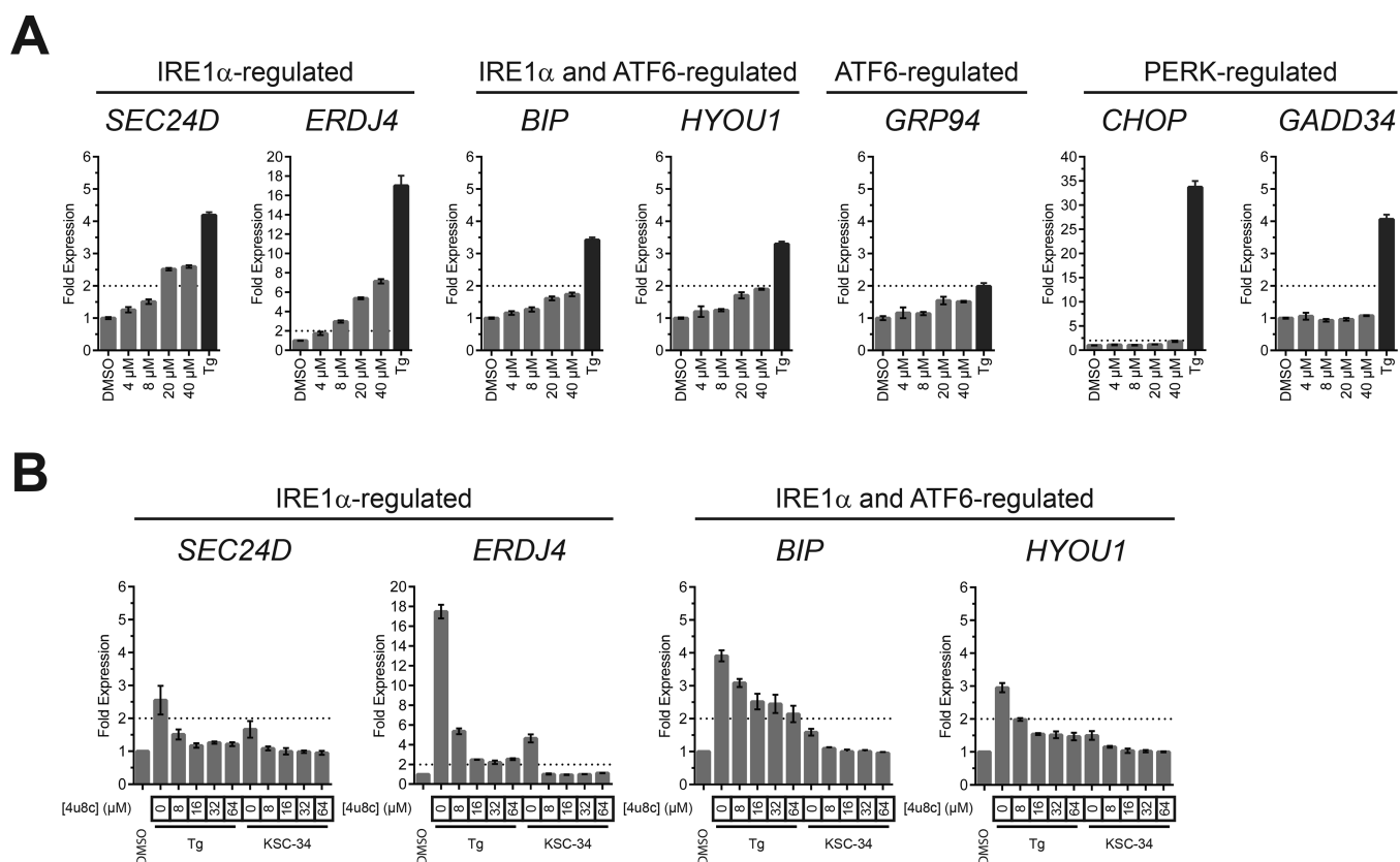
Figure 5. Effects of KSC-34 on cell viability and the unfolded protein response. (A) qPCR analysis of UPR target genes following concentration-dependent treatment of MCF-7 cells with KSC-34 for 3 h at 37 °C. qPCR data are reported as the mean fold change relative to the corresponding DMSO-treated cells \pm SEM from three biological replicates. (B) qPCR analysis of UPR target genes following co-treatment of MCF-7 cells with KSC-34 (20 \mu M) and IRE1 \alpha inhibitor, 4u8c. qPCR data are reported relative to the corresponding DMSO-treated cells \pm SEM from three biological replicates.
